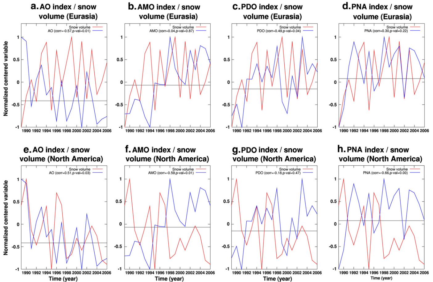
Fig. 4. Annual snow volume over Eurasia (red curves in a., b., c. and d.) and over North America (red curves in e., f., g. and h.) and January to March average of AO (blue cruves in a. and e.), AMO (blue cruves in b. and f.), PDO (blue cruves in c. and g.) and PNA (blue cruves in d. and h.) indices versus time. The time series have been normalized and centered to be plotted at the same scale. On each plot, the gray horizontal line corresponds to the zero in the original climate index time series.
