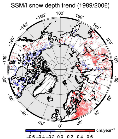
Fig. 3. Map of the annual snow depth trends over the 1989/2006 time span. Only statistically significant trends are shown (i.e. trends with p-value < 0.1).
