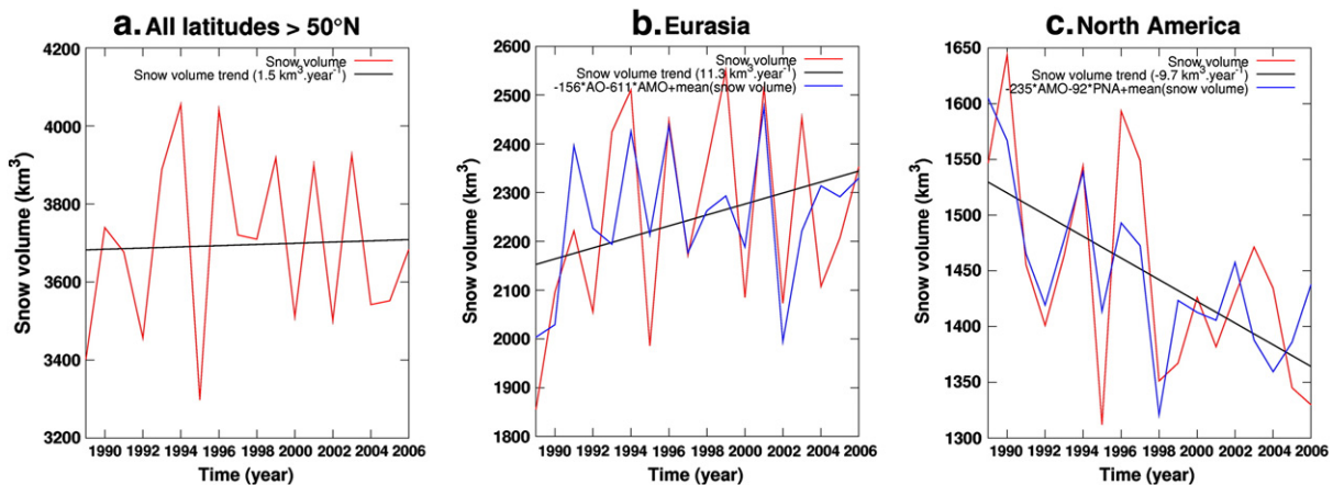
Fig. 2. Annual snow volume from SSM/I data (solid red curve) over the whole study domain (a.), over Eurasia (b.) and over North America (c.). On each plot the black line corresponds to the linear trend and the blue curve corresponds to the linear combination of two climate indices (January to March average) which best correlates with SSM/I snow volume (the mean value of the SSM/I snow volume over the 1989/2006 period has been added to the linear combination).
